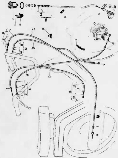
T. IX — CABLES — SPEEDOMETER Page 44
