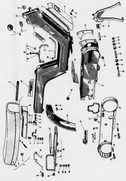
T. IV — CHASSIS — SADDLE — SIDE PROTECTION COVERS Page 22
