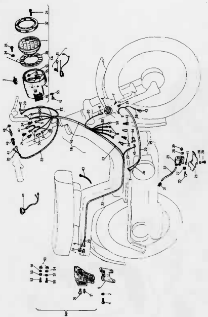
T. VIII — LAMPS AND ELECTRICAL CONNECTIONS Page 40
